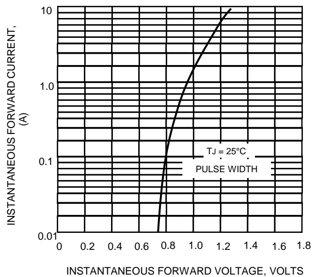
FIG.4-TYPICAL FORWARD CHARACTERISTICS
