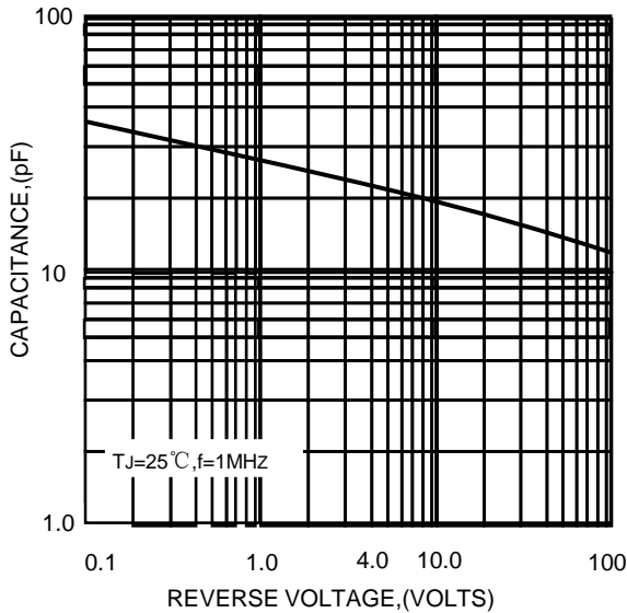
FIG.3-TYPICAL JUNCTION CAPACITANCE
