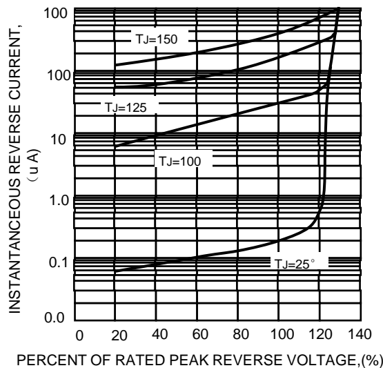
FIG.5-TYPICAL REVERSE CHARACTERISTICS
