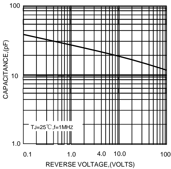
FIG.3-TYPICAL JUNCTION CAPACITANCE
